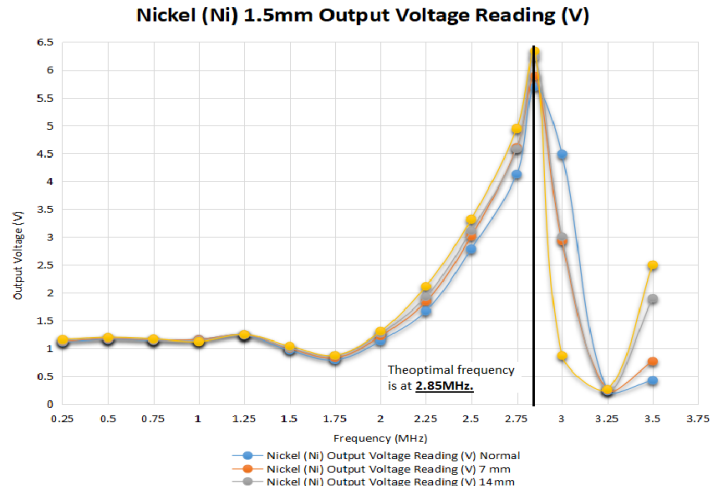
Figure 4.6 The output voltage imperfection of Ni on 1.5mm.
